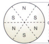
Lateral, n pole sectors on one face only.
